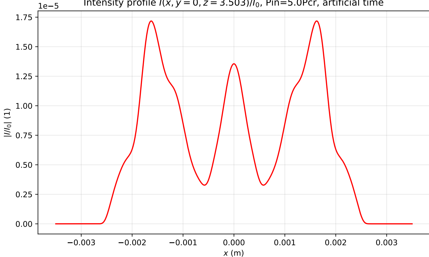
Intensity profile I(x, y = 0, z = 3.503)/I_0 , P_{in}=5.0P_{cr} , artificial time
